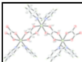
Fig. 1. Part of the polymeric structure of the title compound. Displacement ellipsoids are drawn at the 30% probability level. [Symmetry codes: (i) x, 1-y, 1/2+z ; (ii) 1-x, 1-y, -z ; (iii) 1-x, y, 1/2-z .]
